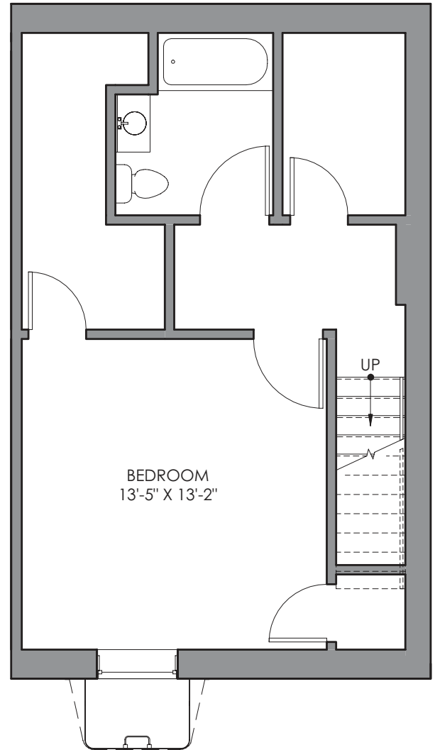
LOWER LEVEL
